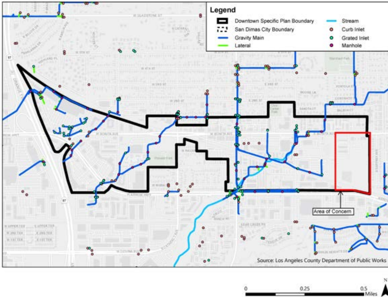
Figure 7.4-2 Storm Drain System Map – Areas of Concern
