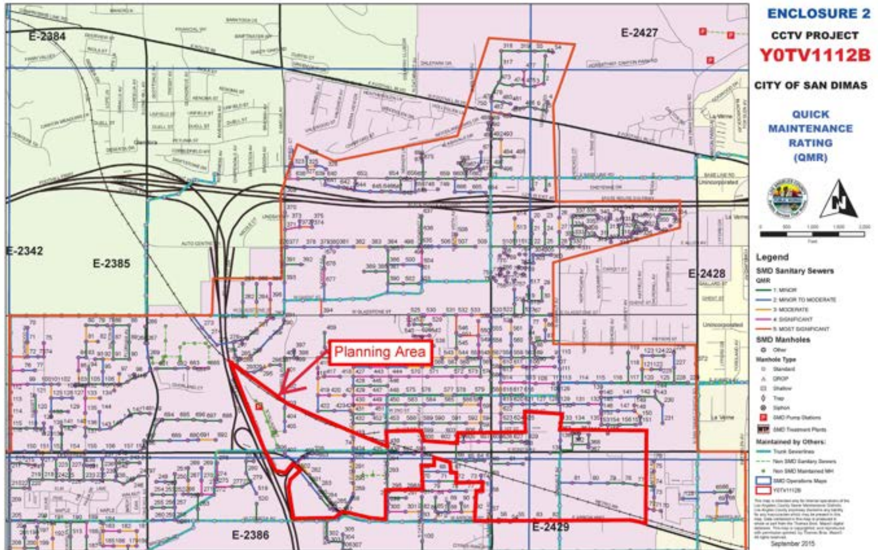
Figure 7.3-2 Sanitary Ratings Map
